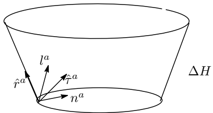
Figure 3.1: This shows spacelike dynamical horizon. \hat{r}^a is normal vector parallel to the dynamics. \hat{r}^a is chosen as orthogonal to \hat{r}^a . l^a is the null normal whose expansion is zero. n^a is the null normal whose expansion is strictly negative. \Delta H is the region between two trapped surface.
